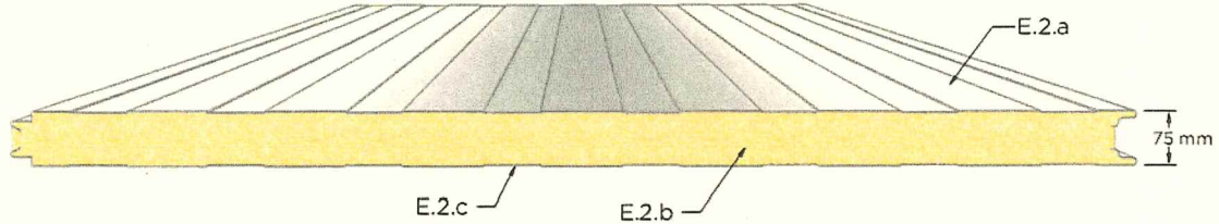
Figure 1. Polyisocyanurate Sandwich Panel - Typical details
